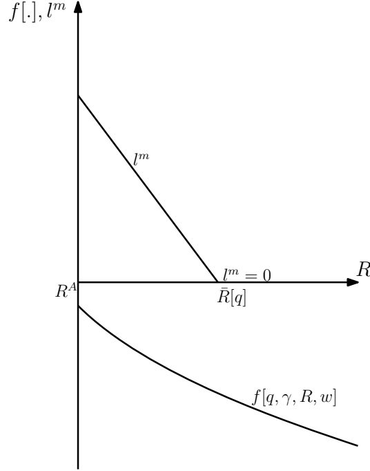
Figure 11: Heterogeneous Societies when q \in (\frac{1}{2}, \tilde{q}) : R^A < \tilde{R}[q]
